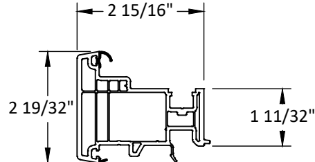
10 MULLION
