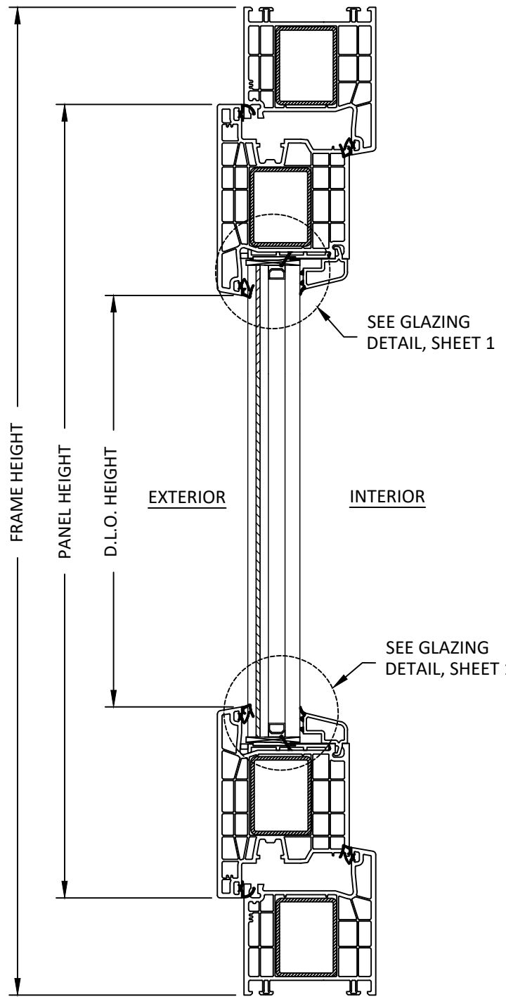
A 4 VERTICAL SECTION OPERABLE WINDOW
