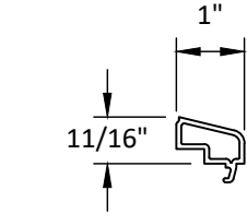
2 I.G. GLAZING BEAD
