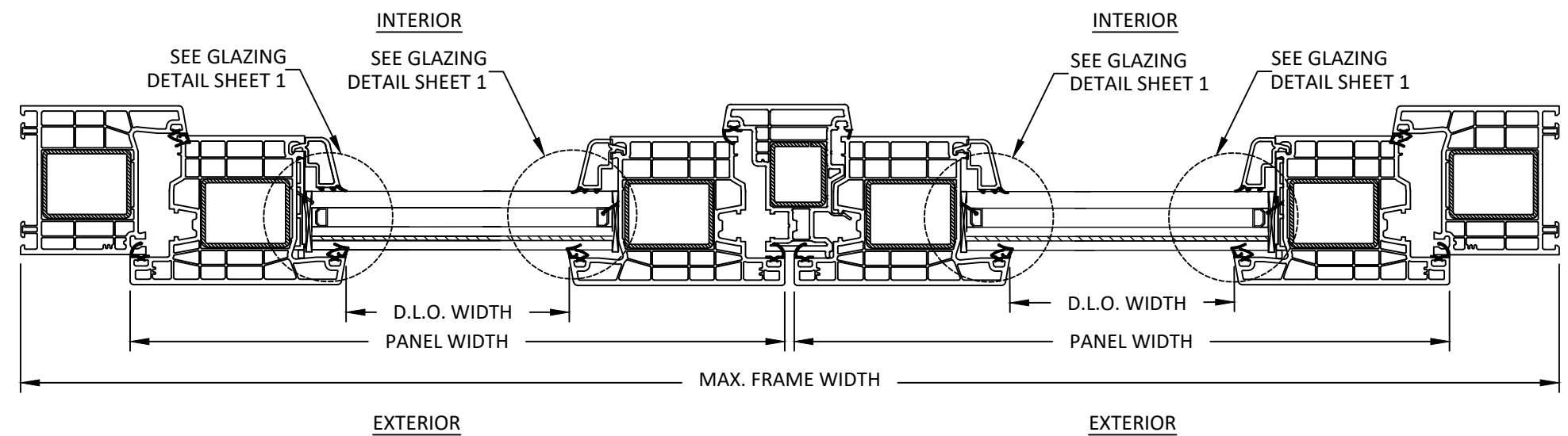
B 4 HORIZONTAL SECTION OPERABLE WINDOW
