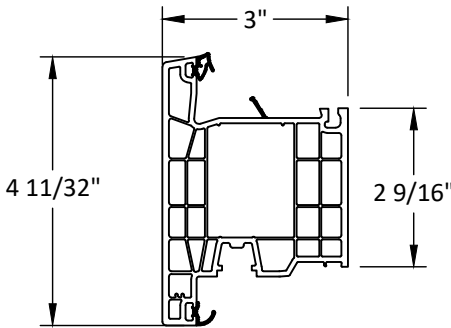
9 MULLION
