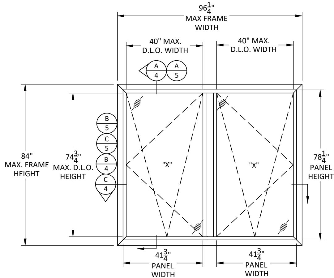
ELEVATION OUTSWING
