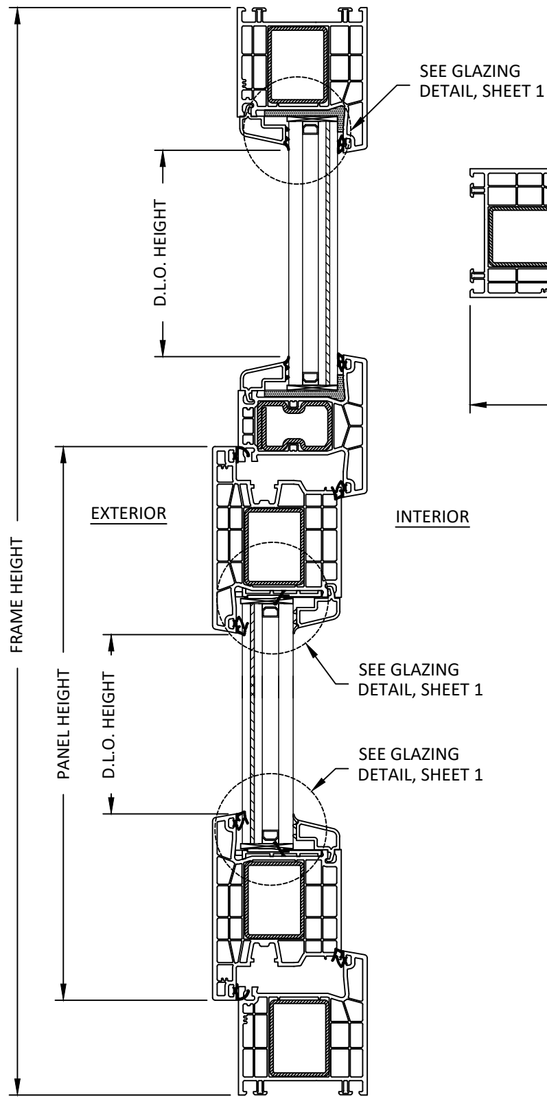
A 5 VERTICAL SECTION OPERABLE FIXED WINDOW
