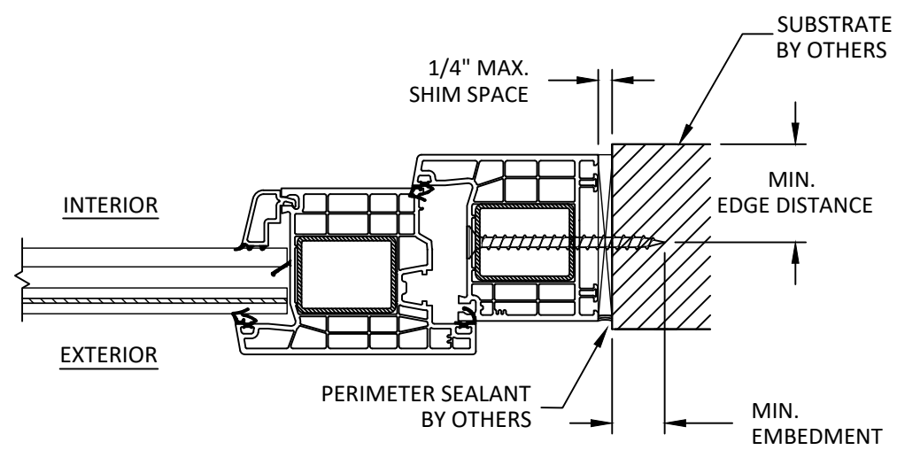
A 6 ANCHOR DETAIL THROUGH FRAME (JAMB)
