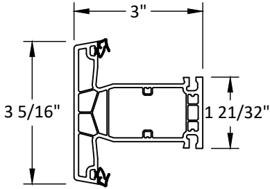
5 MULLION
