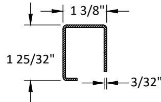
7 REINFORCEMENT
