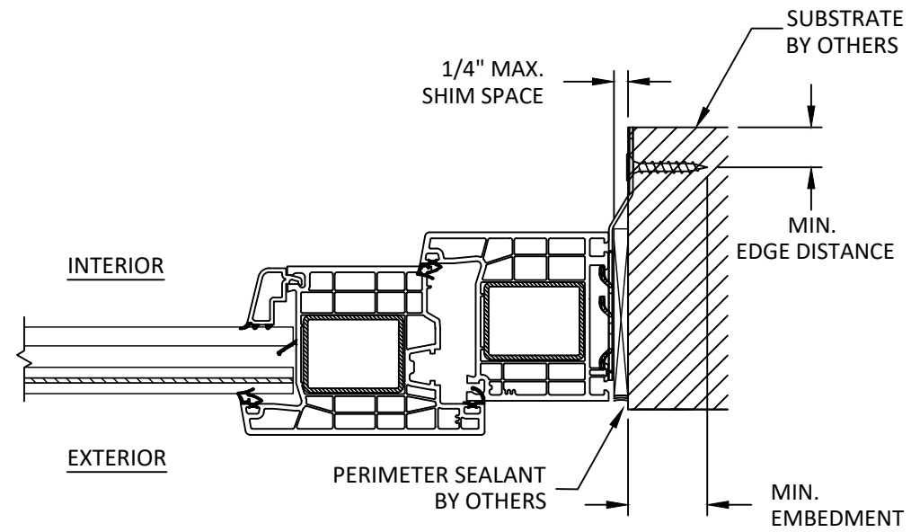
B 6 ANCHOR DETAIL STRAP (JAMB)
